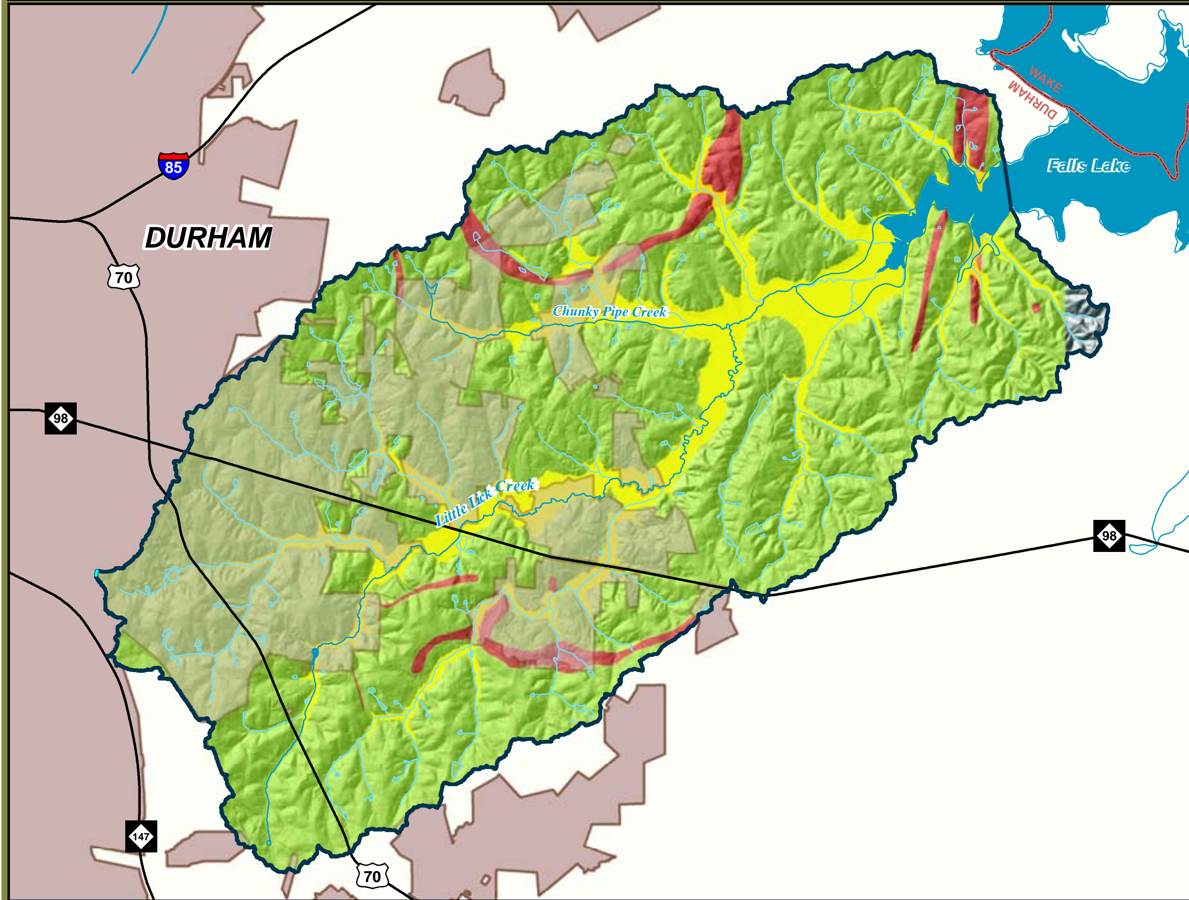
Figure 2: Little Lick Creek Geology
